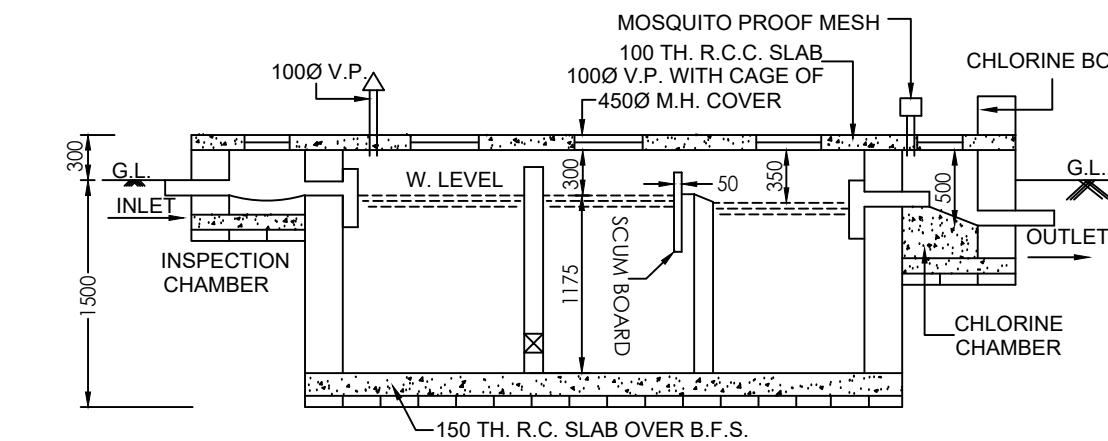
LONG SECTION
