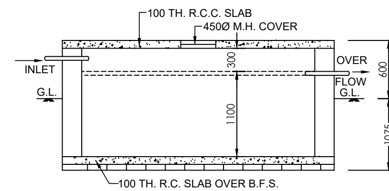
LONG SECTION
